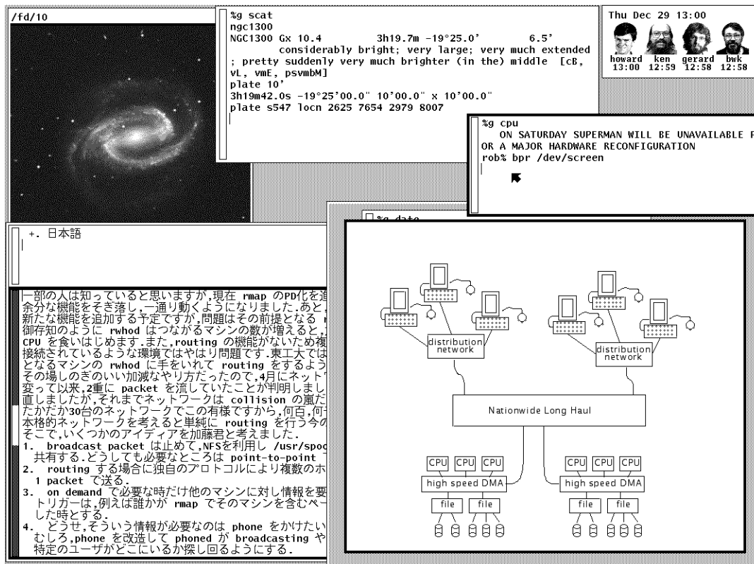
Figure 1. A representative 8\frac{1}{2} screen, running on a NeXTstation under Plan 9 (with no NeXT software). In the upper right, a program announces the arrival of mail. In the top and left are a browser for astronomical databases and an image of a galaxy produced by the browser. In the lower left there is a screen editor, sam [Pike87], editing Japanese text encoded in UTF, and in the lower right an 8\frac{1}{2} running recursively and, inside that instantiation, a previewer for troff output. Underneath the faces is a small window running the command that prints the screen by passing /dev/screen to the bitmap printing utility.
